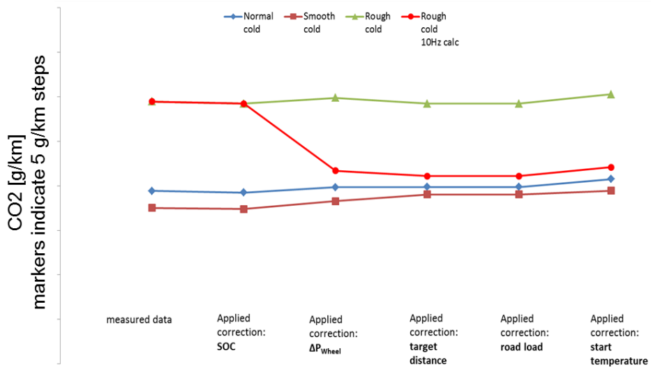
Figure 35: Test results and effects of the correction in the WLTC for diesel vehicle JARI C
