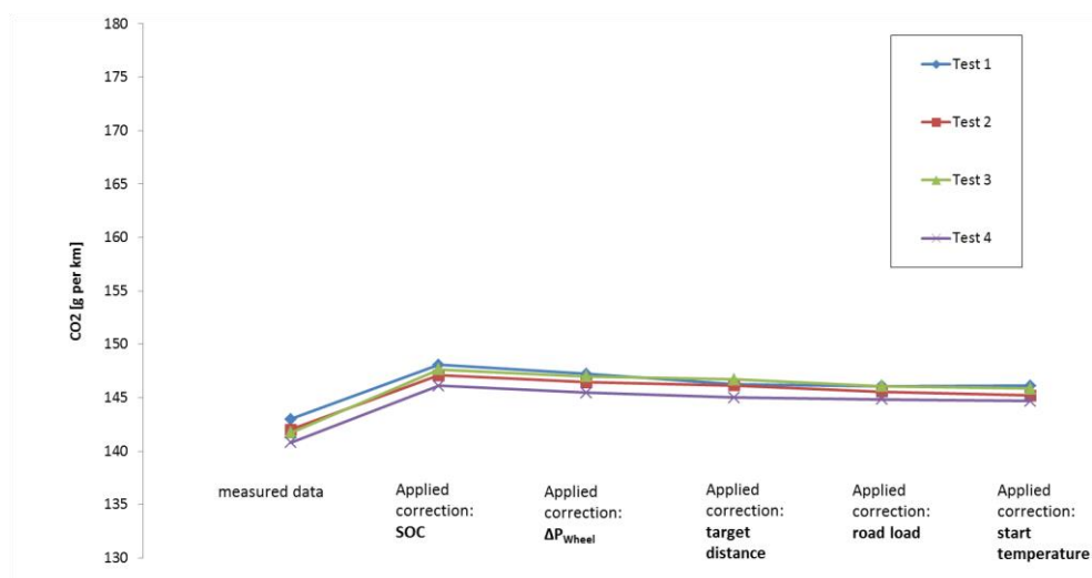
Figure 29: Test results and effects of the correction in the NEDC for vehicle No. 3
