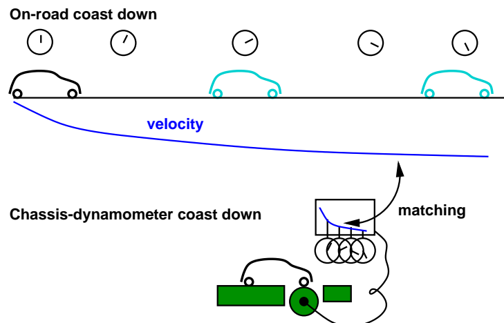
Figure 18 7 : The best guarantee that the road-load settings are appropriate, is if the coast-down test is repeated on the chassis dynamometer, with the same total inertia. The coast-down test on the chassis dynamometer should follow the WLTP test immediately.
