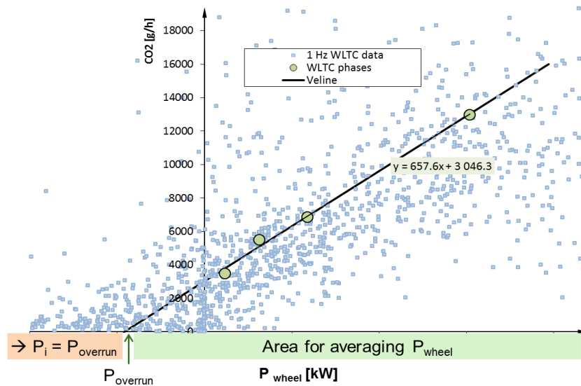
Figure 3: Schematic picture of setting up the Veline equation for a LDV from the chassis dyno test (1 Hz data points only plotted for illustration)
