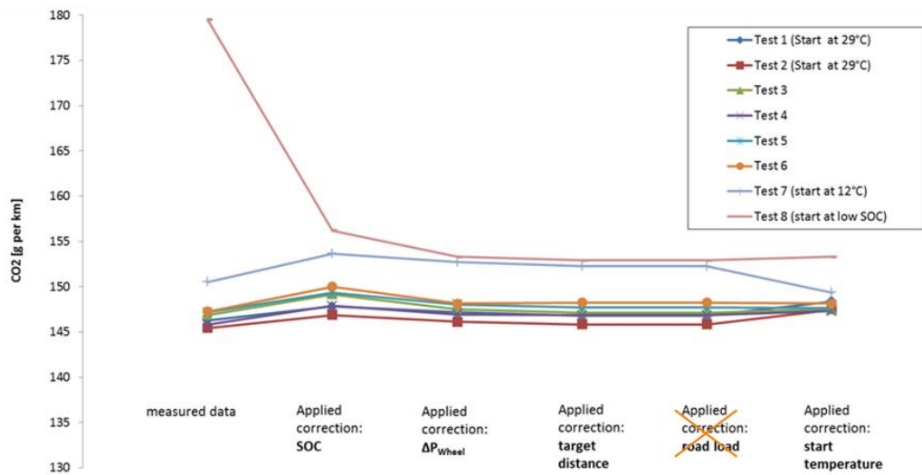
Figure 27: Test results and effects of the correction in the WLTC for diesel vehicle No. 1 (test 1, 2, 7 and 8 were out of WLTP flexibilities to test capability of the correction functions)
