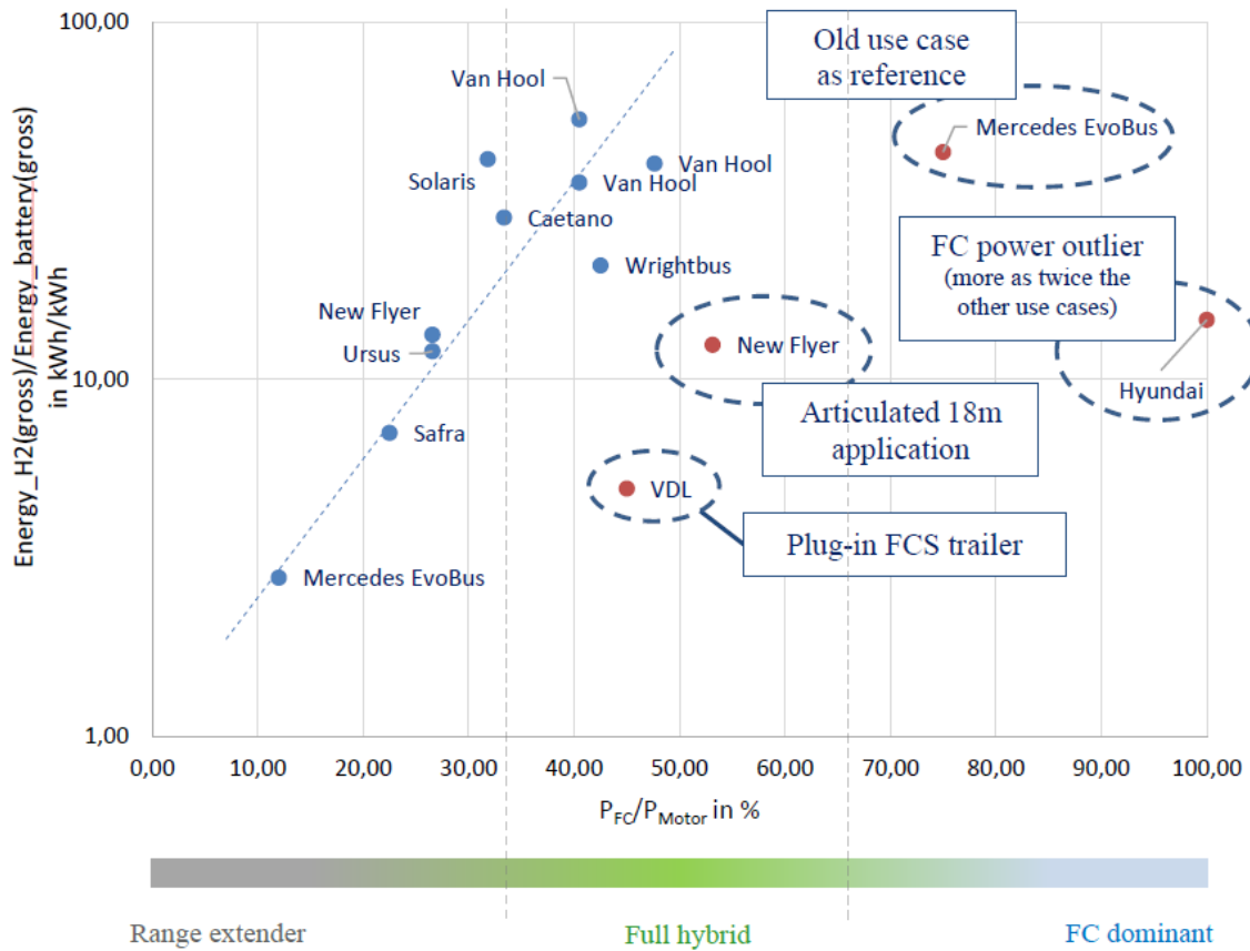
Figure 27: Energy ratio based on powertrain strategy for buses and coaches
