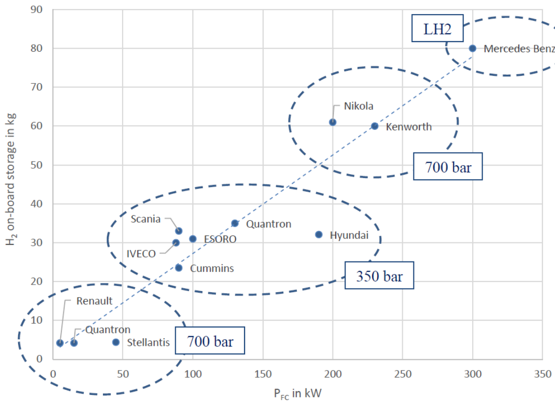
Figure 18: On-board stored H 2 in relation to the installed FC power for commercial vehicles
