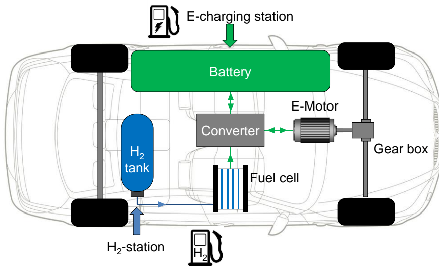
Figure 31: Fuel cell range extender concept [5]
