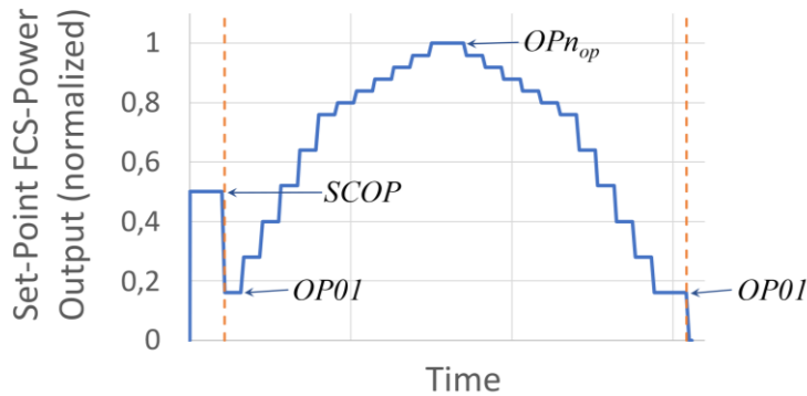
Figure 38: Sequence of operation points in component test
