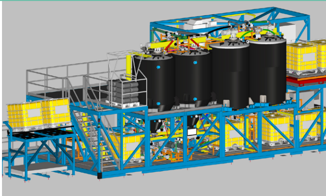
3D model of Recond Oil Standalone Plant for industrial lubricant oil reconditioning
