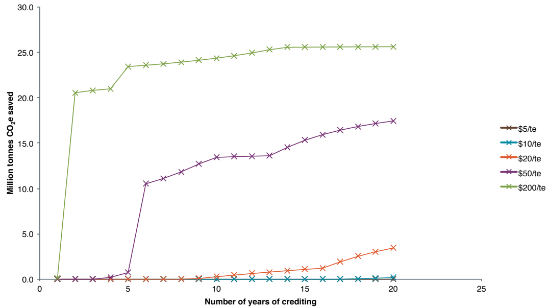
Figure 3.13. Emissions reductions at varying numbers of years for which credit support is active, at varying marginal abatement cost, excluding non-additional projects
