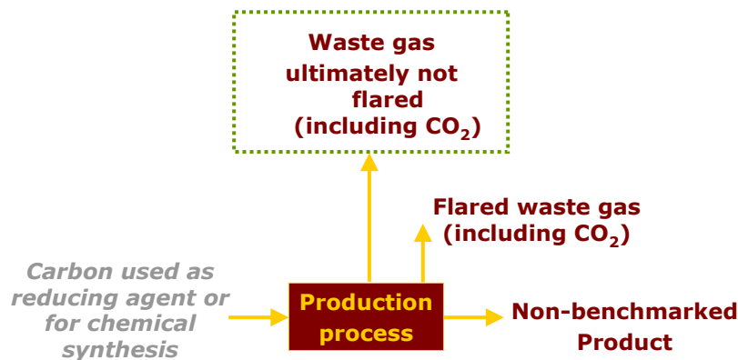
Figure 4 Emission of waste gases outside the boundaries of a product benchmark. The green dashed line shows the boundaries of a process emissions sub-installation 5
