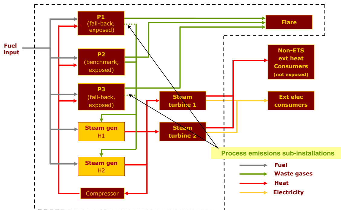
Figure 10 Example 1 – Waste gases from non-benchmarked products (P1 and P3) are included in a process emissions sub-installation 7 . The allocation related to these process
