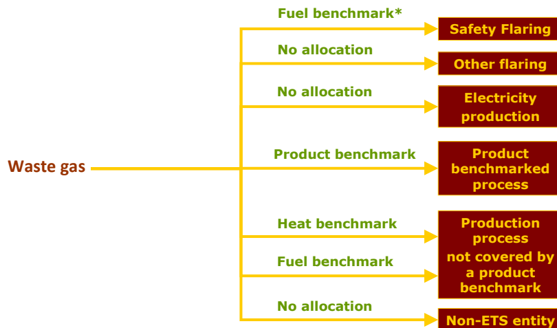
Figure 5 Allocation for the consumption of waste gases (part C in Figure 2); *Safety flaring only receives allocation based on a fuel benchmark in case the flared waste gas is produced outside the boundaries of a product benchmark
