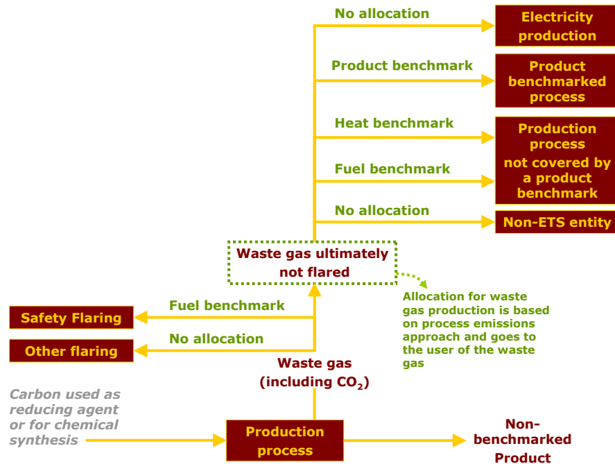
Figure 7 Overview of allocation in case of production of waste gases outside the boundaries of a product benchmark. The green dashed line indicates the boundaries of a process emissions sub-installation
