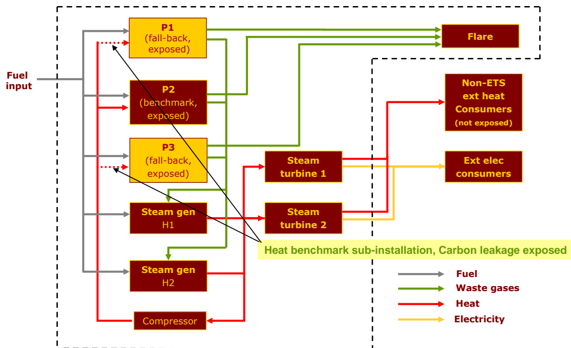
Figure 11 Example 1 – P1 and P3 receive allocation for consumed heat that was partially produced using waste gases; Raw material flows are not shown (e.g. carbon used as reducing agent or chemical synthesis).
