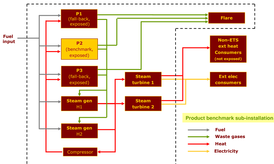
Figure 9 Example 1 – Waste gases produced by P2 (highlighted process) are included in the product benchmark P2; Raw material flows are not shown (e.g. carbon used as reducing agent or chemical synthesis).
