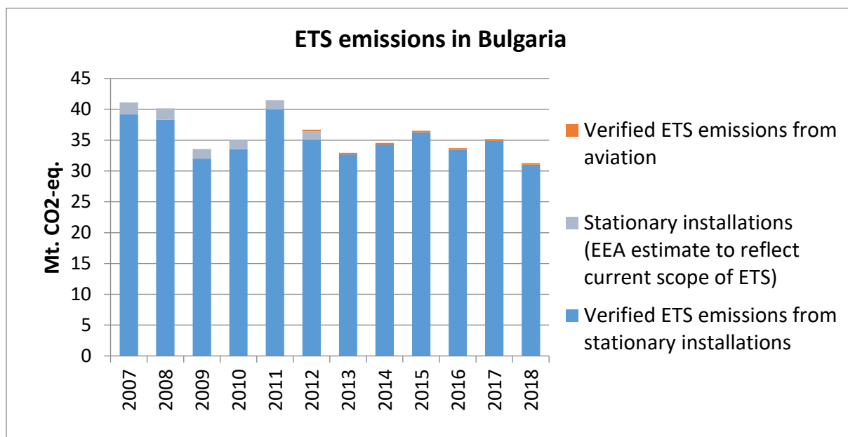
Figure 3: ETS emissions 2005-2018 (Mt CO 2 -eq). 3
