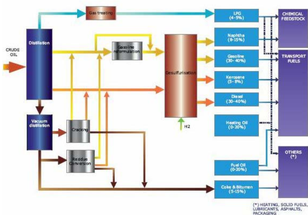
Figure 5: Overview of the oil refinery process. Source: Europa
